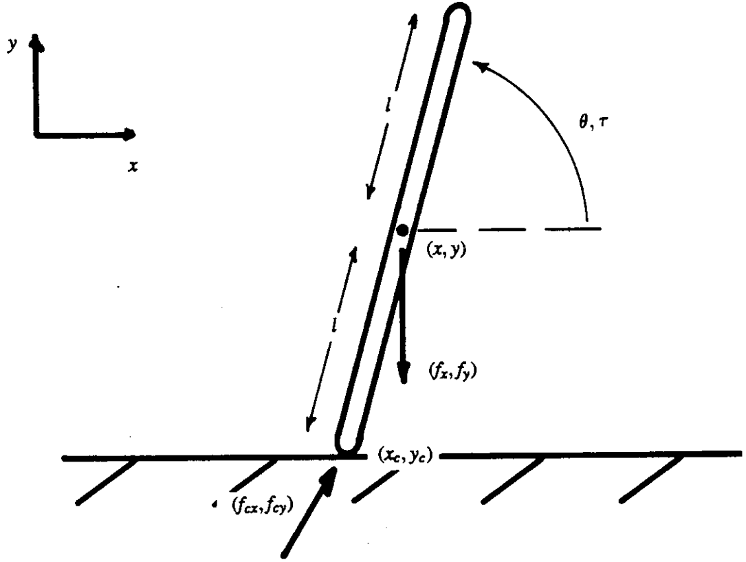
Figure 1: A rigid rod on a frictional surface.
