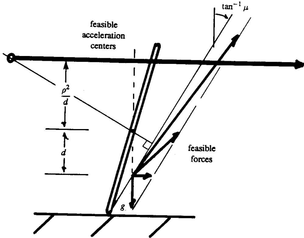
Figure 3: The locus of feasible acceleration centers.
